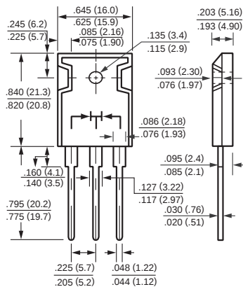
TO-247
