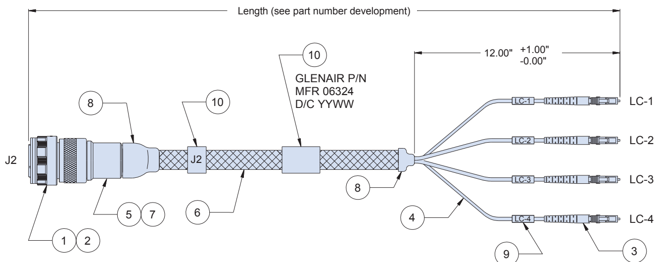
Connection Diagram
