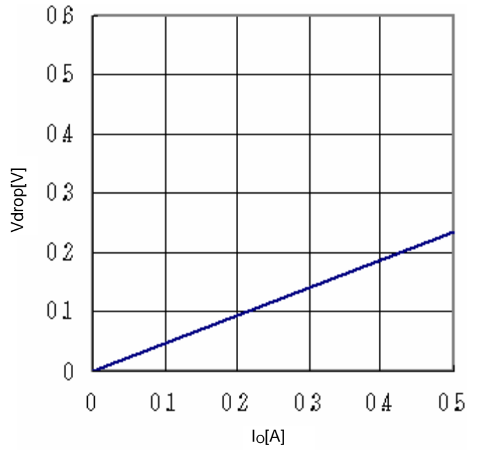
Fig.25 Minimum dropout Voltage 6 ( V_{CC}=12V , T_a=25^\circ C )
