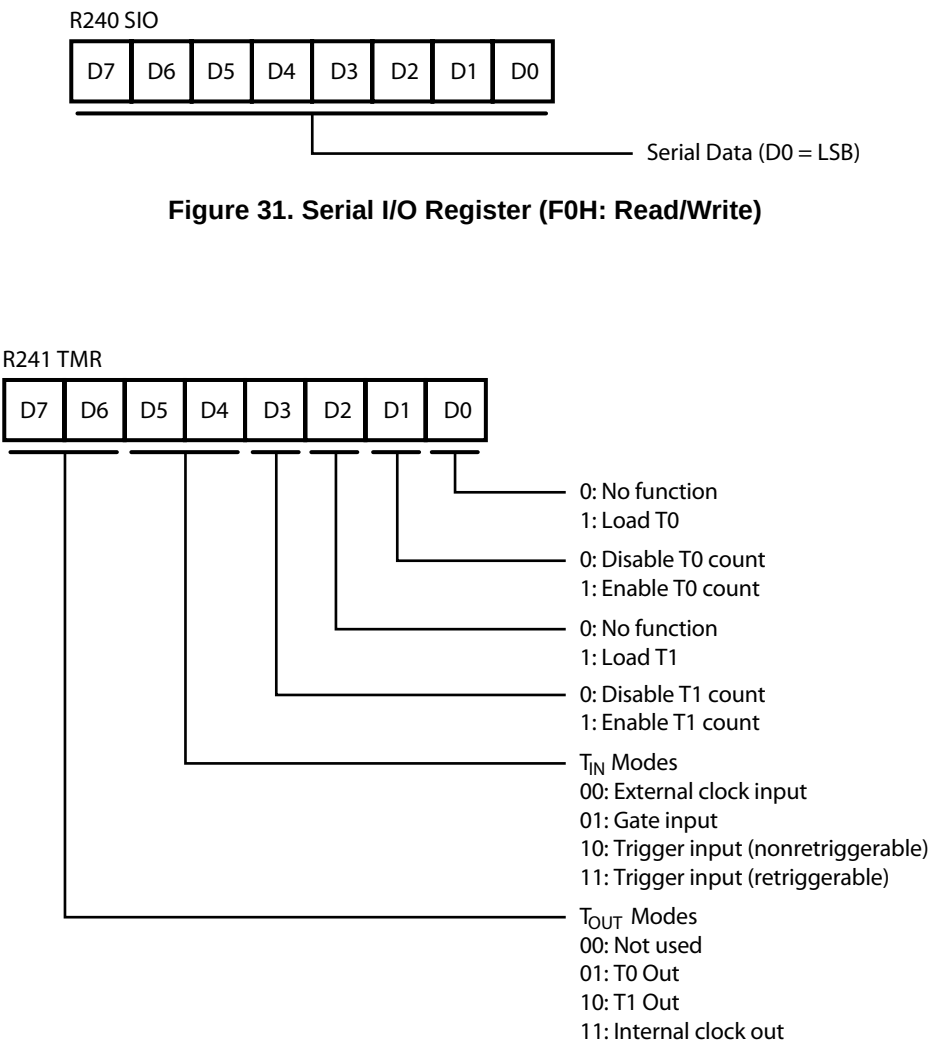
Figure 32. Timer Mode Register (F1H: Read/Write)
