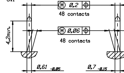
View X 5:1
