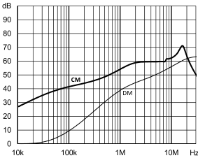
FN 9266 Standard Type 2 A
