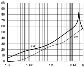
FN 9266 Standard Type 10 A
