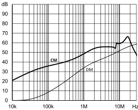
FN 9266 Standard Type 4 A
