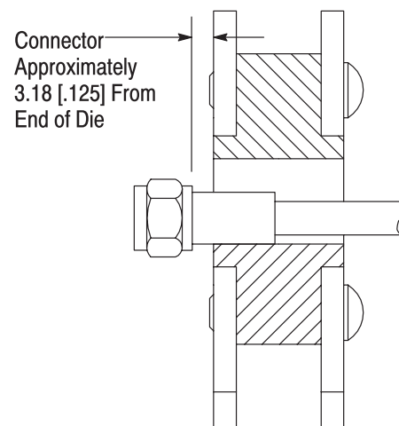
Crimping Ferrule
