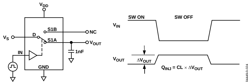
Figure 23. Charge Injection
