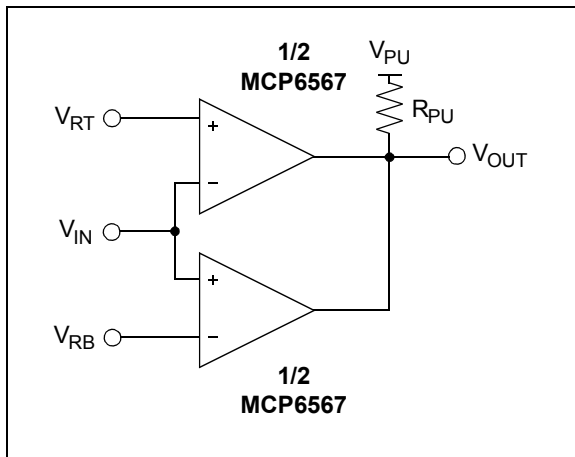
FIGURE 4-13: Windowed Comparator.
