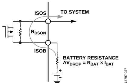
Figure 44. Discharge Current Sensing Through Battery Isolation FET
