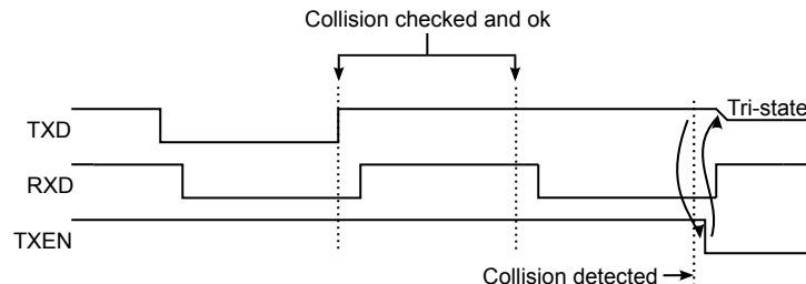
Figure 32-18. Collision Detected
