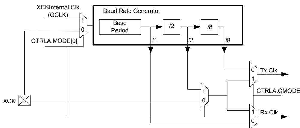
Figure 32-3. Clock Generation
