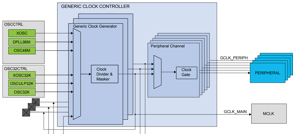
Figure 17-1. Device Clocking Diagram
