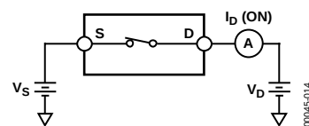
Figure 14. On Leakage
