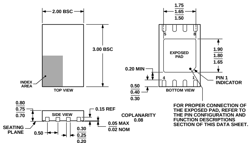
Figure 24. 8-Lead Lead Frame Chip Scale Package [LFCSP_WD] 3 mm x 2 mm Body, Very Very Thin, Dual Lead (CP-8-4)
