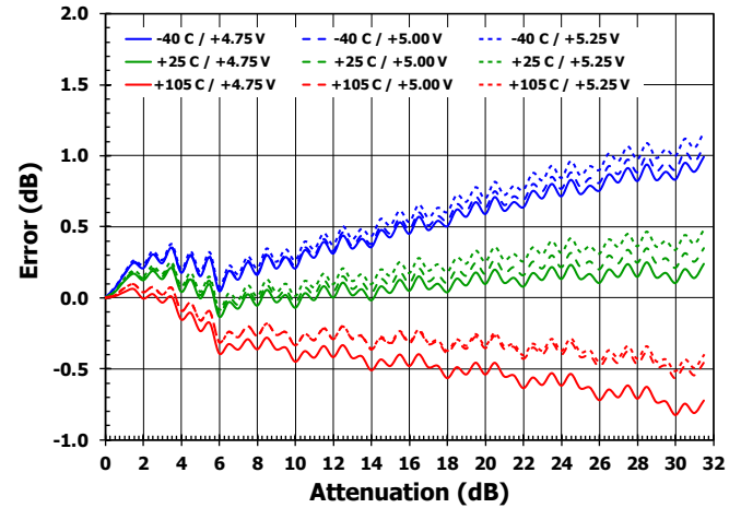
Figure 14. Step Accuracy vs. Attenuation over Temperature and Voltage [2.65 GHz]
