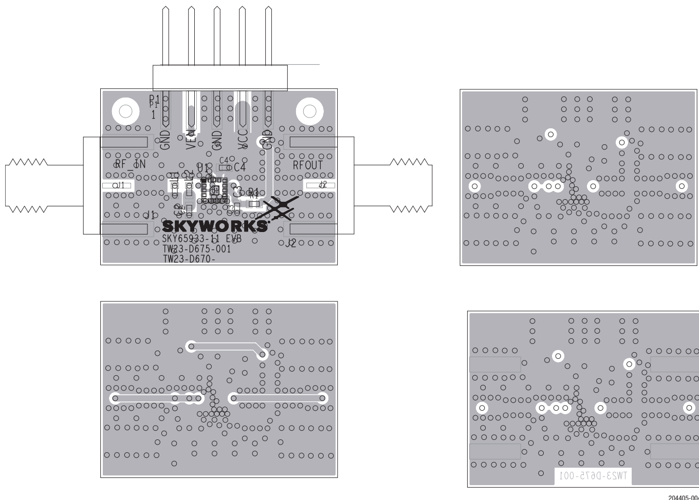
Figure 4. SKY65933-11 Evaluation Board Assembly Diagram
