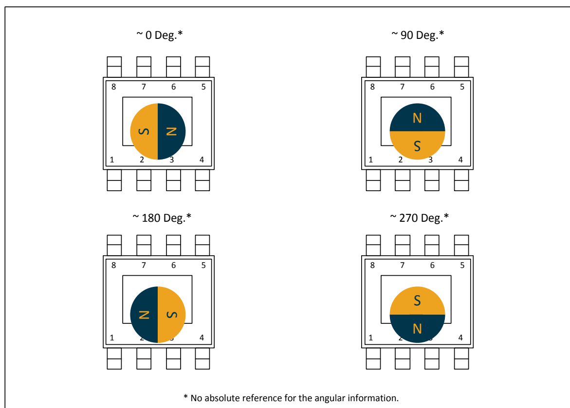
fig. 31 - SOIC-8 Angle Detection
