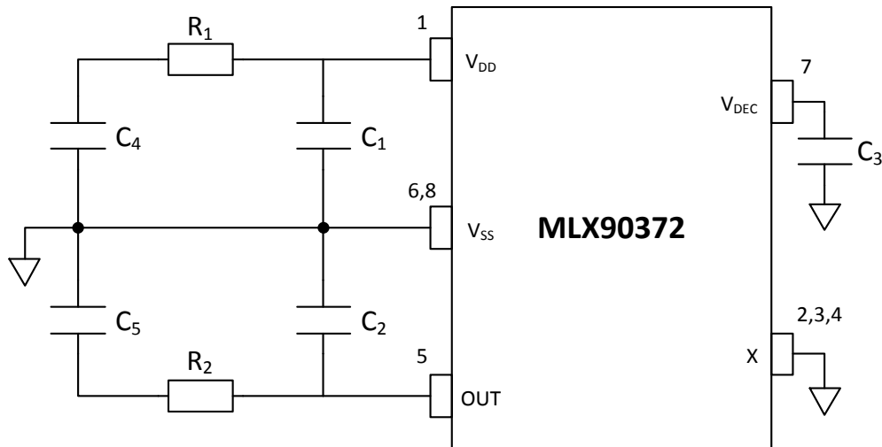
fig. 24 - Recommended wiring for the MLX90372 in SOIC-8 package
