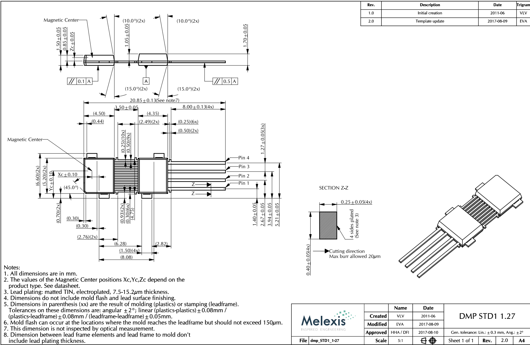
fig. 37 - DMP-4 STD1 1.27 Package Outline Drawing
