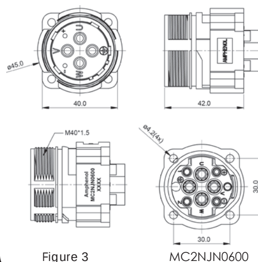
Receptacle, 90° fixed, Checkmate™
