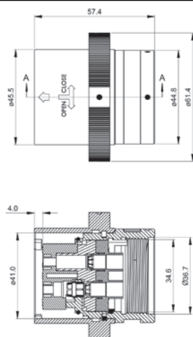
Plug, straight, Checkmate™
