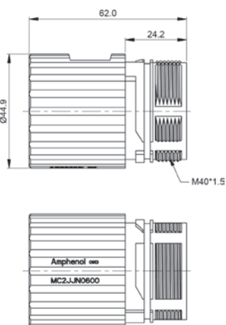
Receptacle extension, straight, Checkmate™
