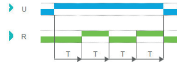
Function D - Symmetrical flashing (OFF Start)
