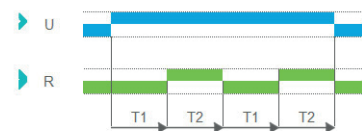
Function L - Recycler (OFF Start)
