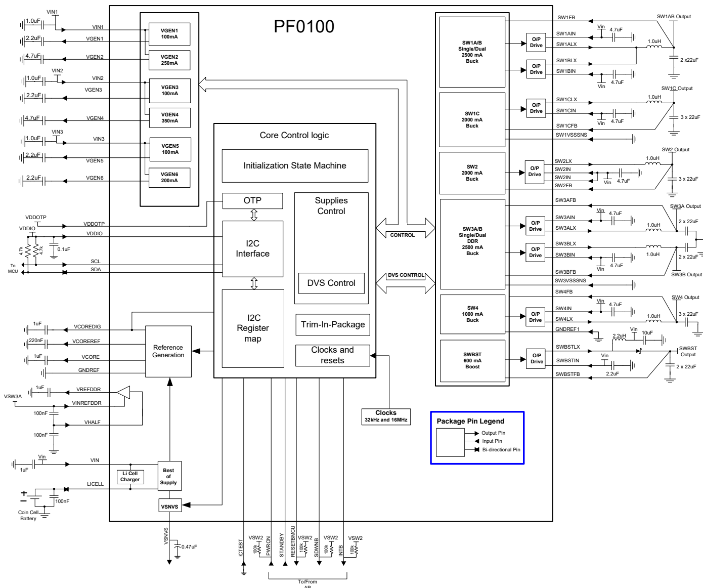
Figure 35. Typical application schematic
