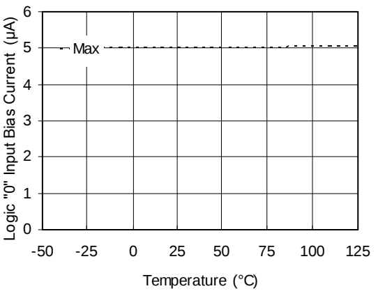
Figure 29A. Logic “0” Input Bias Current vs. Temperature
