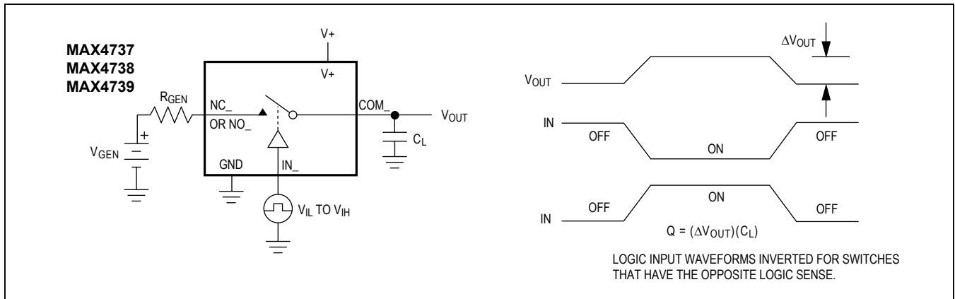
Figure 4. Charge Injection
