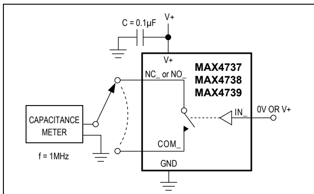
Figure 6. Channel Off-/On-Capacitance
