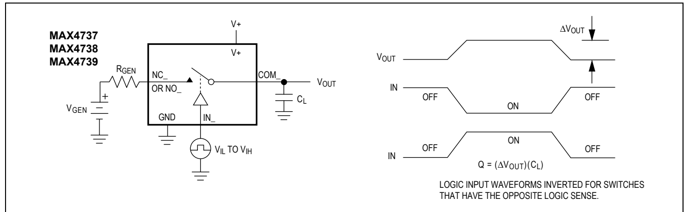
Figure 4. Charge Injection
