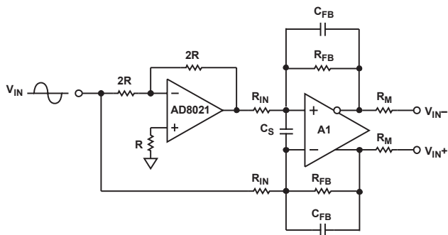
Figure 53. Single-Ended-to-Differential Conversion
