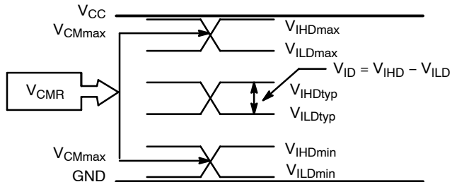
Figure 16. V_{CMR} Diagram
