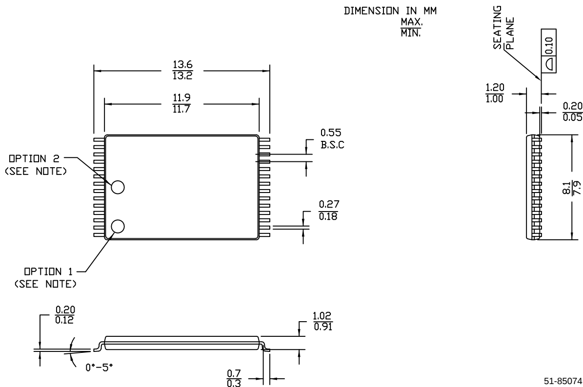
Figure 10. 28-pin Reverse TSOP 1 (8 × 13.4 mm), 51-85074
