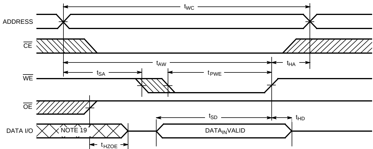
Figure 5. Write Cycle No. 1 (WE Controlled) [16, 17, 18]
