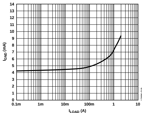
Figure 19. Ground Current ( I_{GND} ) vs. Load Current ( I_{LOAD} ), V_{OUT} = 1.8\text{ V}
