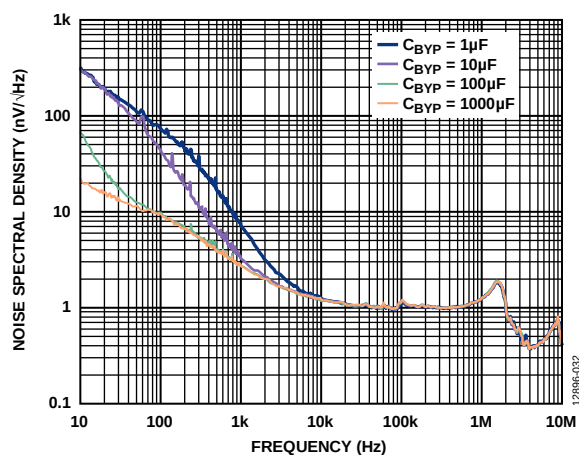
Figure 30. Noise Spectral Density vs. Frequency at Various Values of C_{\text{BYP}}
