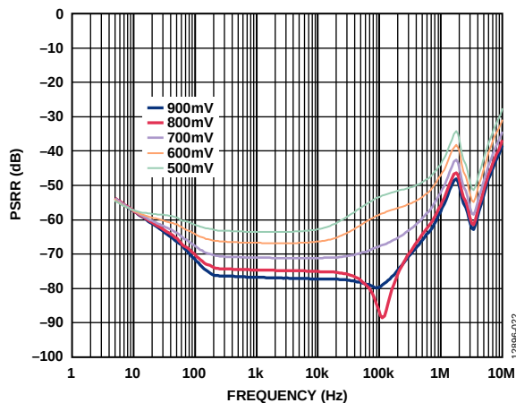
Figure 22. PSRR vs. Frequency at Various Headroom Voltages, V_{OUT} = 3.3\text{ V} , 2 A Load
