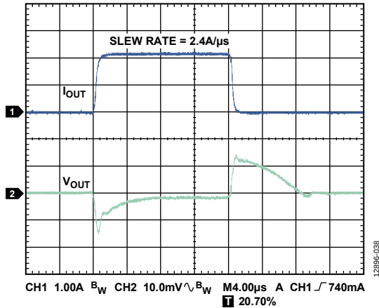
Figure 36. Load Transient Response, I_{LOAD} = 100\text{ mA} to 2\text{ A} , V_{OUT} = 1.8\text{ V} , V_{IN} = 2.5\text{ V} , C_{OUT} = 22\text{ μF} , Channel 1 = I_{OUT} , Channel 2 = V_{OUT}
