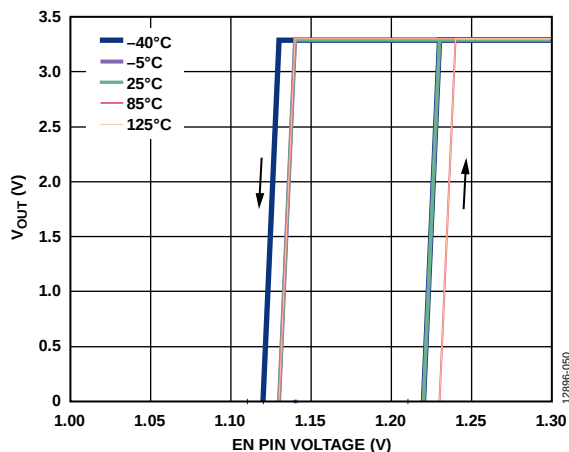
Figure 48. Typical V OUT Response to EN Pin Operation
