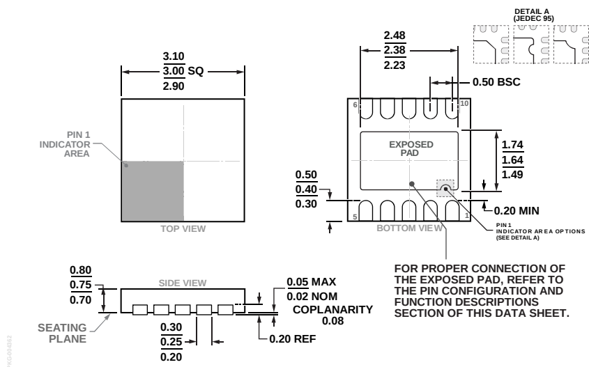
Figure 64. 10-Lead Lead Frame Chip Scale Package [LFCSP] 3 mm x 3 mm Body and 0.75 mm Package Height (CP-10-9)
