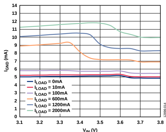
Figure 14. Ground Current ( I_{GND} ) vs. Input Voltage ( V_{IN} ) at Various Loads in Dropout, V_{OUT} = 3.3\text{ V}
