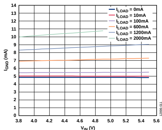
Figure 11. Ground Current ( I_{GND} ) vs. Input Voltage ( V_{IN} ) at Various Loads, V_{OUT} = 3.3\text{ V}
