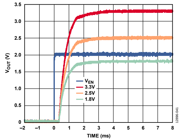
Figure 39. V_{OUT} Start-Up Time After V_{EN} Rising at Various Output Voltages, V_{IN} = 5\text{ V} , C_{BYP} = 1\text{ μF}
