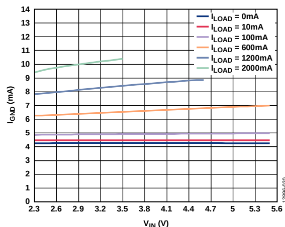
Figure 20. Ground Current ( I_{GND} ) vs. Input Voltage ( V_{IN} ) at Various Loads, V_{OUT} = 1.8\text{ V}
