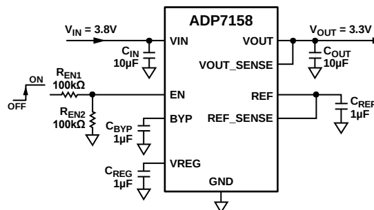
Figure 51. Typical EN Pin Voltage Divider
