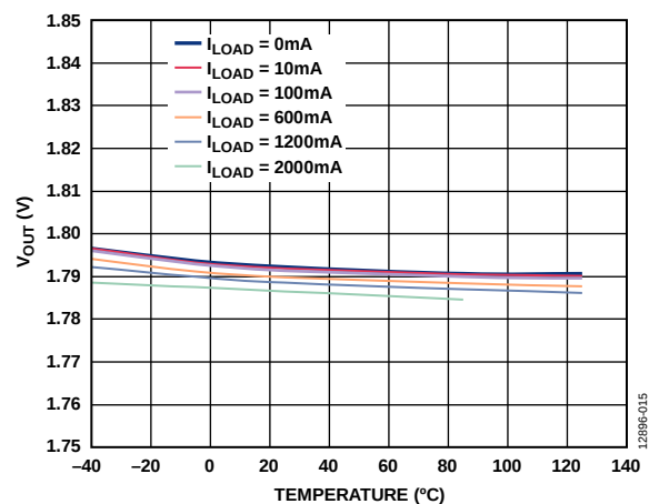
Figure 15. Output Voltage ( V_{OUT} ) vs. Temperature at Various Loads, V_{OUT} = 1.8\text{ V}
