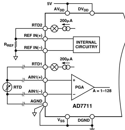
Figure 19. 4-Wire RTD Application with the AD7711
