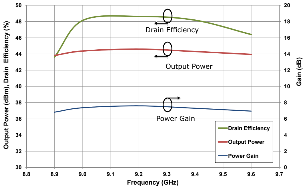
Figure 2. - Typical Large Signal Response V_{DD} = 40\text{ V} , I_{DQ} = 150\text{ mA} , P_{IN} = 37\text{ dBm} T_{case} = 25^\circ\text{C} , Pulse Width = 100\text{ }\mu\text{s} , Duty Cycle = 10 %
