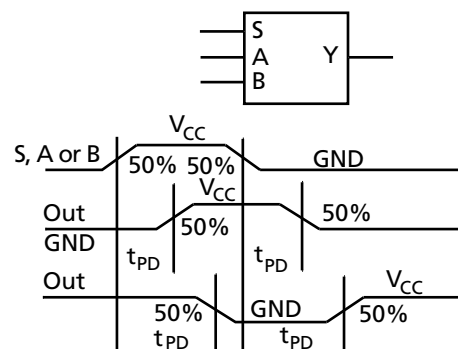
Figure 1-17 • C-Cell Delays
