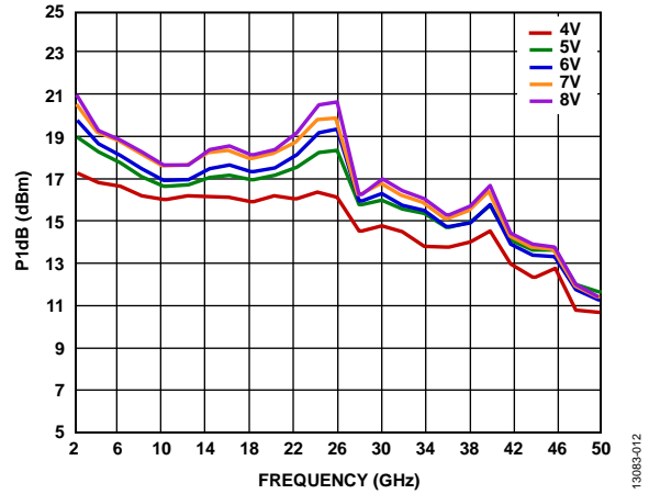
Figure 18. P1dB vs. Frequency at Various Supply Voltages (For V_{DD} = 4V, V_{GG2} = 1.4V ; for V_{DD} = 5V, V_{GG2} = 1.4V ; for V_{DD} = 6V, V_{GG2} = 2V ; for V_{DD} = 7V, V_{GG2} = 3V ; for V_{DD} = 8V, V_{GG2} = 3.6V )
