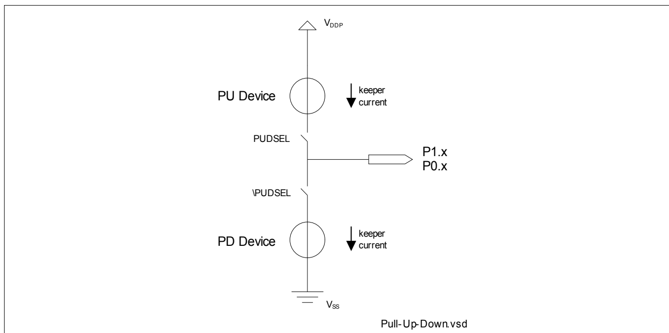
Figure 38 Pull-Up/Down Device
