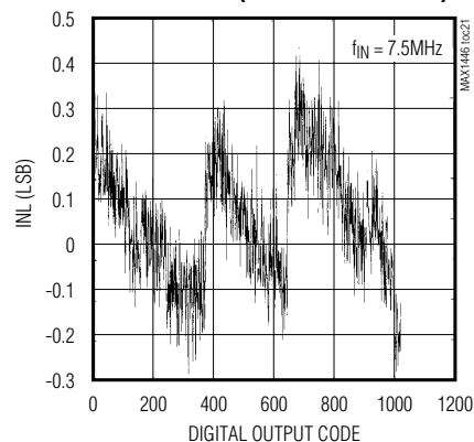
INTEGRAL NONLINEARITY vs. DIGITAL OUTPUT CODE (BEST STRAIGHT LINE)
