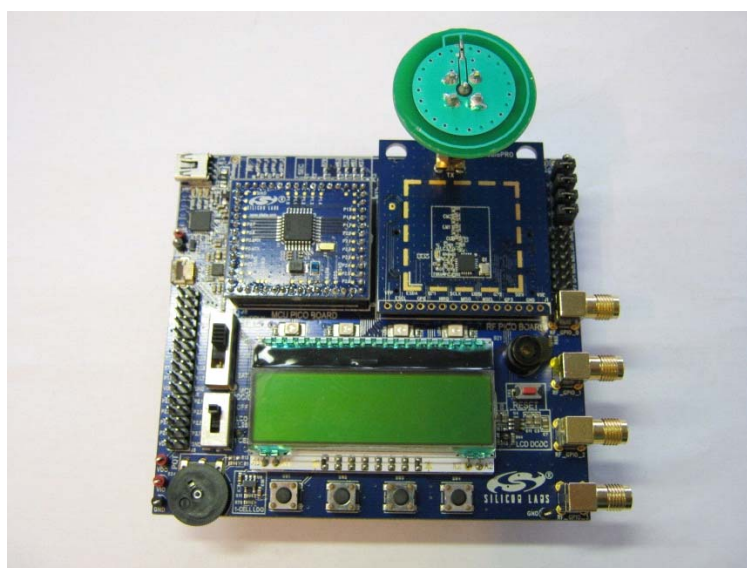
Figure 1. Typical Measurement Configuration—Antenna Board, Pico Board, and Wireless Motherboard
