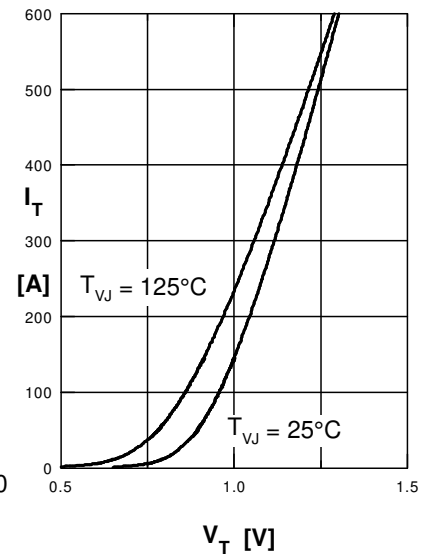
Fig. 9 Forward characteristics
