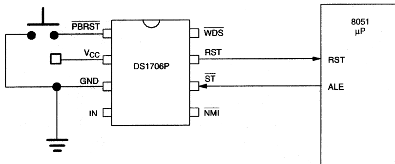
PUSH-BUTTON RESET Figure 2
