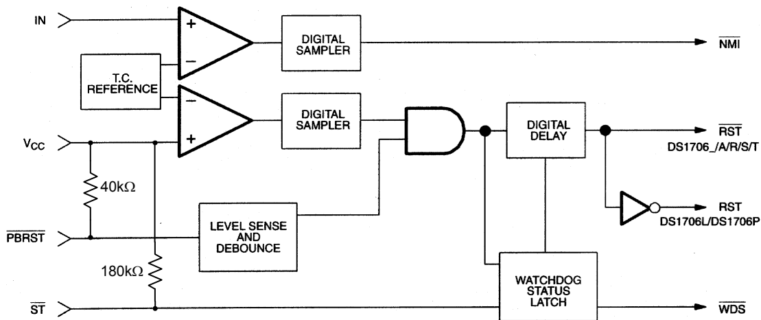
PUSH-BUTTON RESET Figure 2
