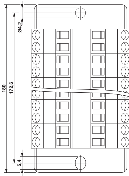
Dimensional drawing
