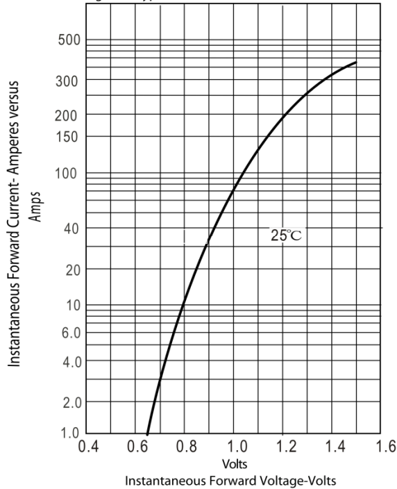
Figure.1-Typical Forward Characteristics
