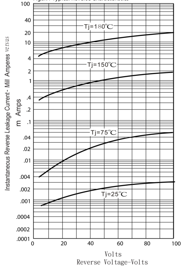
Figur.4-Typical Reverse Characteristics
