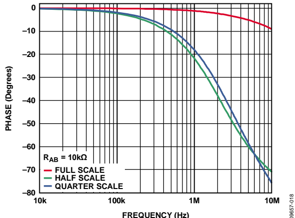
Figure 18. Normalized Phase Flatness vs. Frequency
