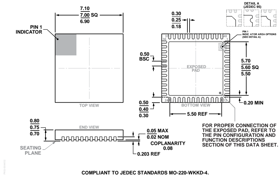
COMPLIANT TO JEDEC STANDARDS MO-220-WKKD-4. Figure 135. 48-Lead Lead Frame Chip Scale Package [LFCS] 7 mm × 7 mm Body and 0.75 mm Package Height (CP-48-13) Dimensions shown in millimeters
