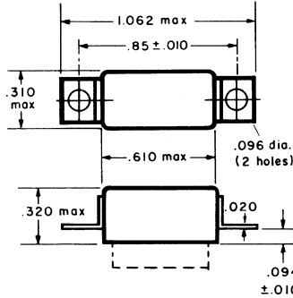
End Bracket
