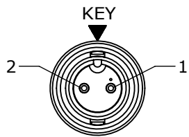
FACE VIEW
