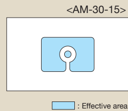
Amorphous Photosensor Pattern Shape Example
