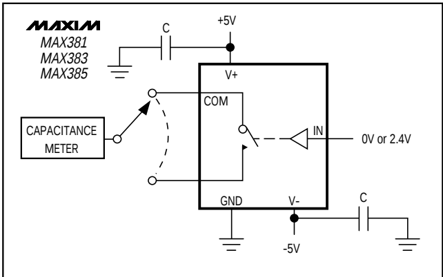
Figure 8. Channel-On Capacitance
