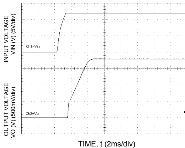
Fig-38. Typical Start-up Using Input Voltage (VIN = 12V, Io = Io,max).
