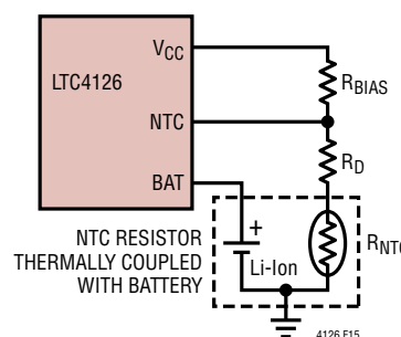
Figure 15. NTC Thermistor Connection with Desensitizing Resistor R_D
