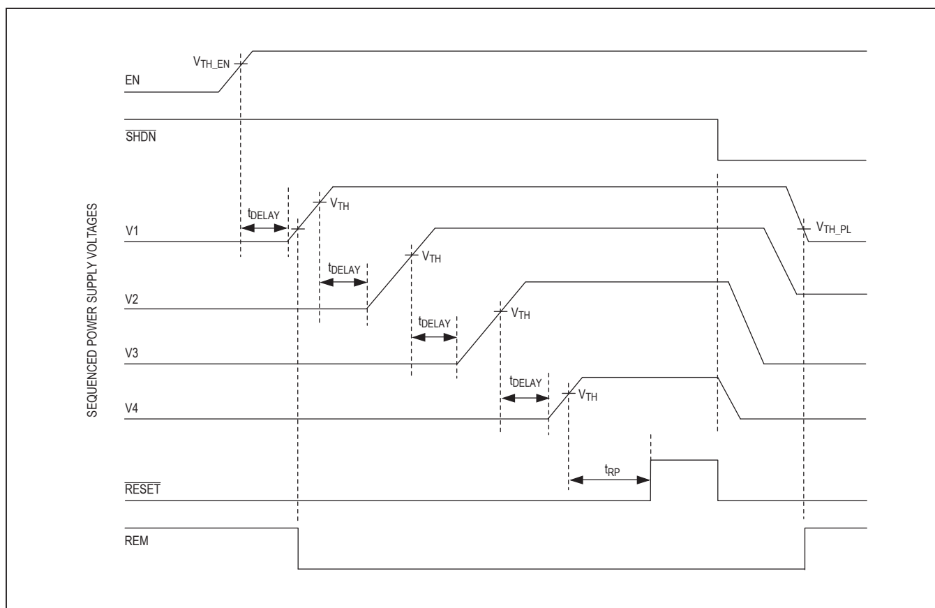
Figure 2. Sequencing Timing Diagram with Reverse Order Power-Down Using \overline{\text{SHDN}} . See the Typical Application Circuit ( Figure 1 ).
