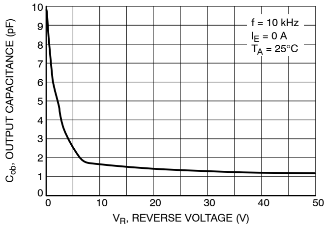
Figure 4. Output Capacitance
