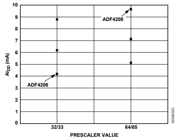
Figure 21. ADF4206/ADF4208 A_{LDD} vs. Prescaler Value (RF1)
