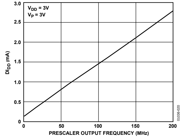
Figure 20. I_{DD} vs. Prescaler Output Frequency RF1 and RF2 (All Models)
